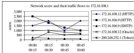
Fig. 14. Users and respective protocols observed in a certain resource
