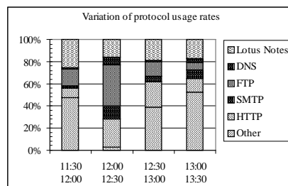
Fig. 9. Departmental network usage rates
