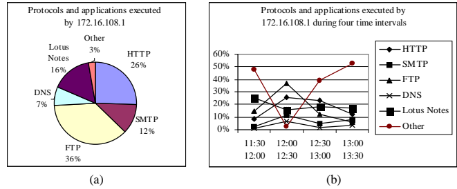
Fig. 5. Example of graphs depicting protocol usage rates
