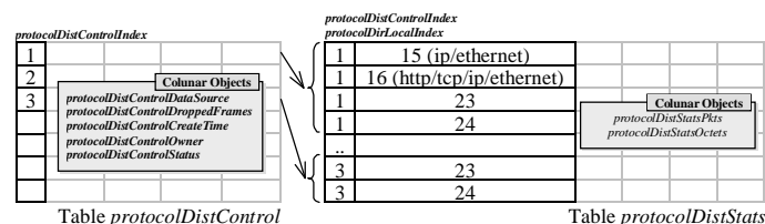
Fig. 7. protocolDist group tables
