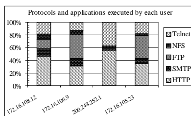
Fig. 15. Users and the protocols executed by them
